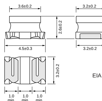
LQH4N/LQN4N Type
